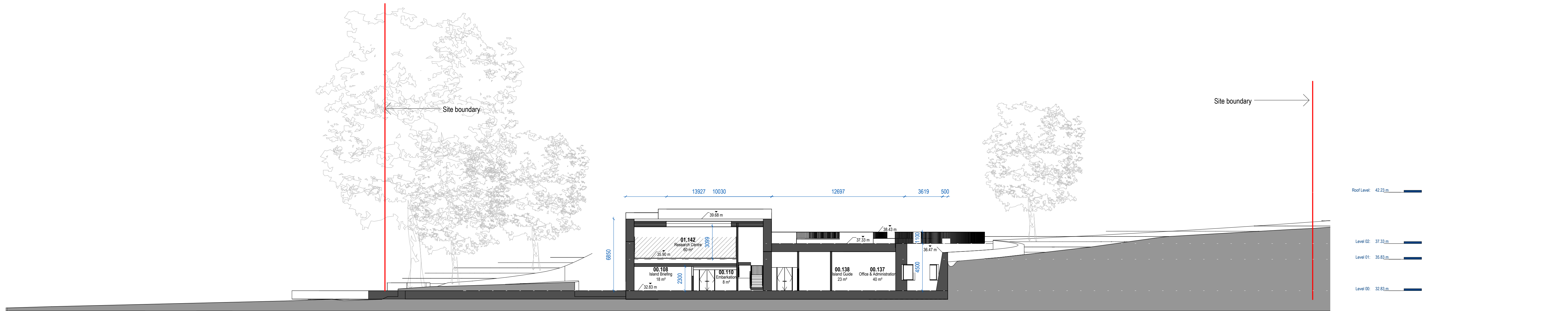
2 Proposed Section BB Scale - 1 : 200
